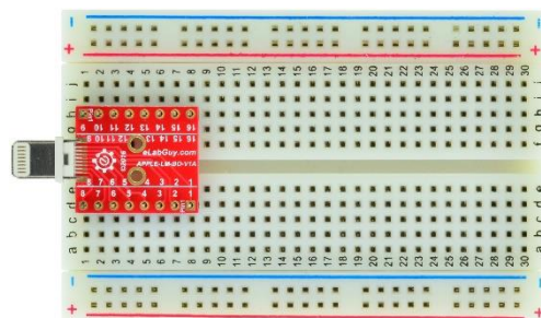
Figure 2: Example of connecting the APPLE-LM-BO-V1A on a breadboard
