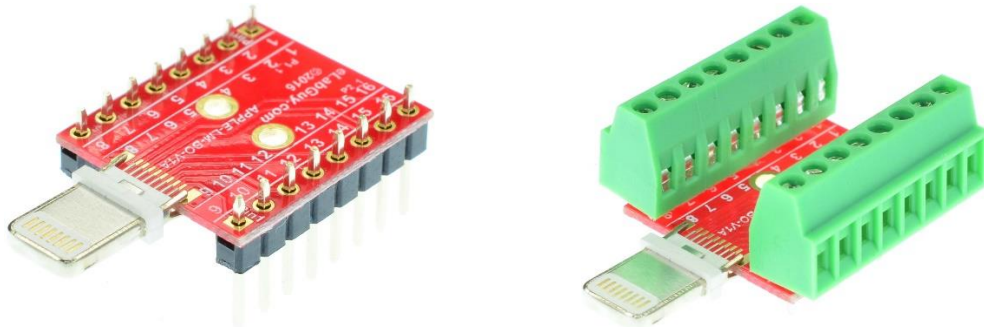
Figure 3: APPLE-LM-BO-V1A Various connections
